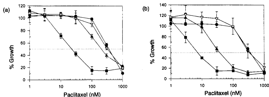
Figure 2. Modulation of MDA-435/LCC6-MDR sensitivity to paclitaxel by MDR reversal taxane 2 (a) and 7 (b) at three different concentrations (circle, 0 \mu M; square, 1 \mu M; triangle, 0.1 \mu M; inverted triangle, 0.01 \mu M).
