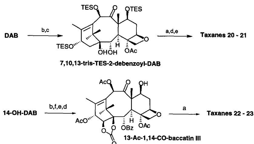
Scheme 2. (a) \text{RCO}_2\text{H} , DCC, DMAP, \text{CH}_2\text{Cl}_2 , room temperature; (b) TESCl, imidazole, DMF, room temperature; (c) Red-Al®, THF, 0 °C; (d) HF-pyridine, pyridine/ \text{CH}_3\text{CN} , 0 °C to room temperature; (e) \text{Ac}_2\text{O} , DMAP, \text{CH}_2\text{Cl}_2 , room temperature; (f) \text{COCl}_2 , pyridine, \text{CH}_2\text{Cl}_2 , 0 °C. TES = triethylsilyl; Troc = 2,2,2-trichloroethoxy carbonyl
