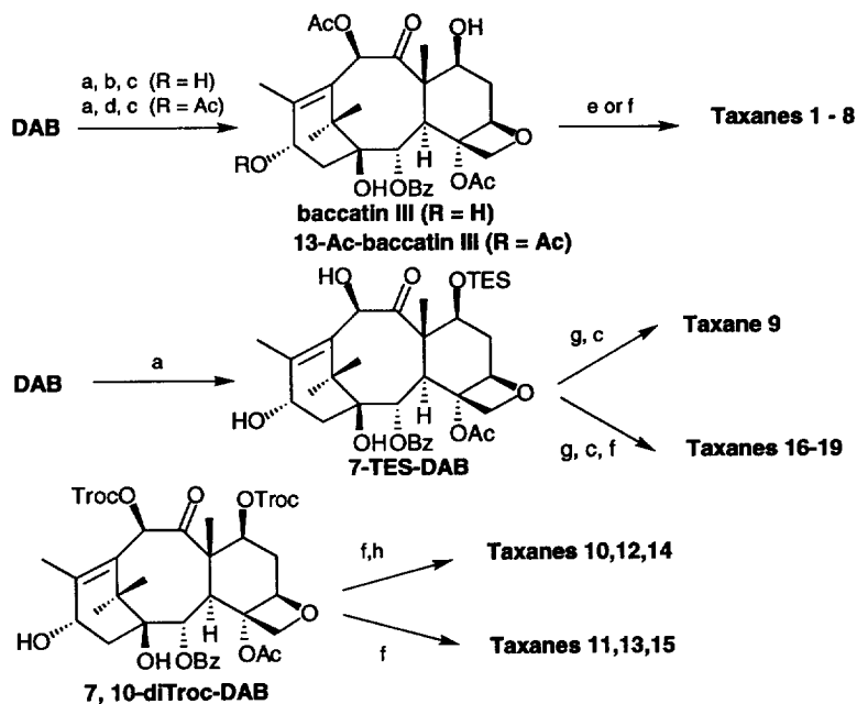
Scheme 1. (a) TESCl, pyridine, room temperature; (b) LiHMDS, AcCl, THF, -40^{\circ}\text{C} ; (c) HF-pyridine, pyridine/ \text{CH}_3\text{CN} , 0^{\circ}\text{C} to room temperature; (d) \text{Ac}_2\text{O} , DMAP, \text{CH}_2\text{Cl}_2 , room temperature; (e) \text{RCOCl} , \text{Et}_3\text{N} , DMAP, \text{CH}_2\text{Cl}_2 , room temperature; (f) \text{RCO}_2\text{H} , DCC, DMAP, \text{CH}_2\text{Cl}_2 , room temperature; (g) N -hydroxysuccinimide ester of \text{RCO}_2\text{H} , LiHMDS, THF, -40^{\circ}\text{C} ; (h) Zn, AcOH/MeOH, 70^{\circ}\text{C} . TES = triethylsilyl.
